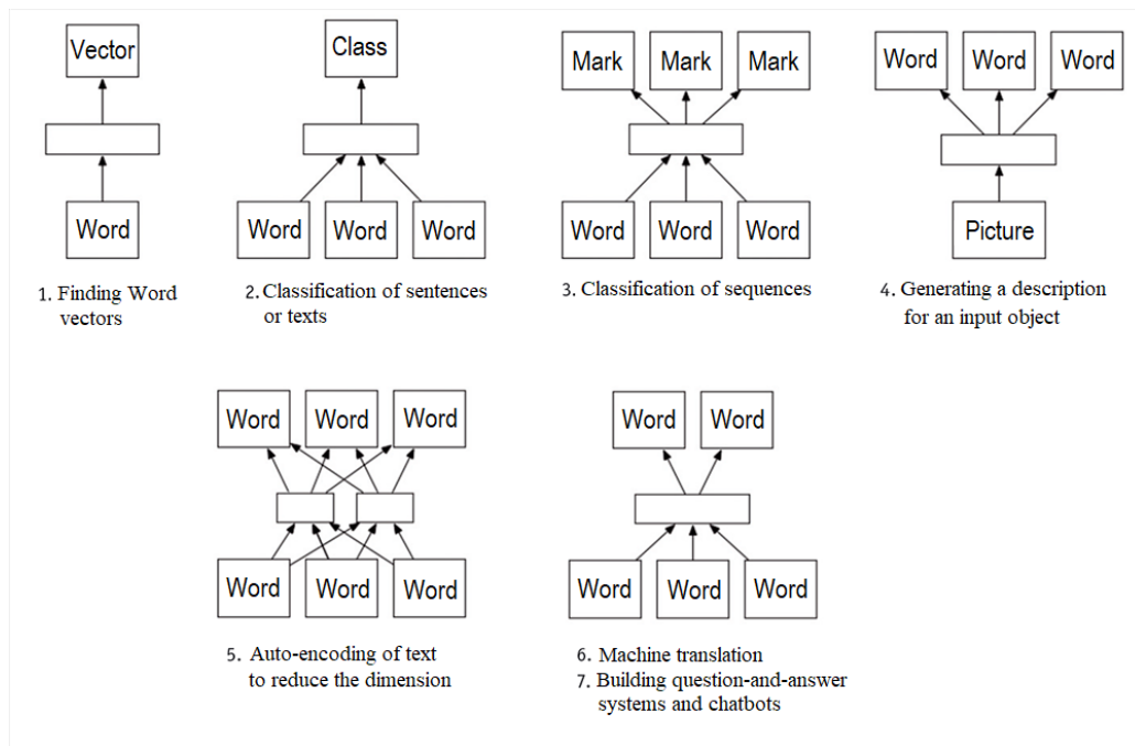
Figure 2. The architecture of a neural network for text processing [2]
